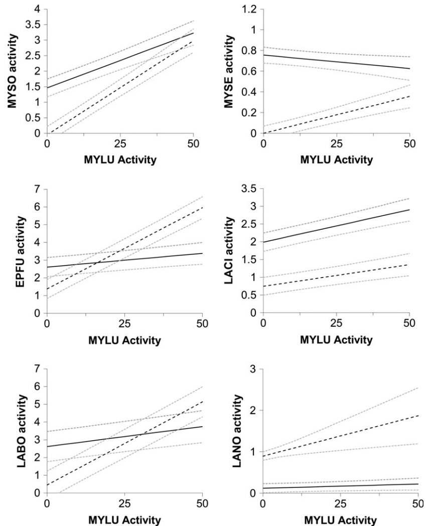
Figure 3 Predicted effect of activity of the predominant bat species (little brown bat, Myotis lucifugus , MYLU) on activity (detections/hr) of 6 other bat species detected in Ft. Drum, New York, USA based on parameter coefficients from top-ranked models. Predictive plots are divided into time periods prior to (solid line, 2003–2007) and following (dashed line, 2008–2011) white-nose syndrome (WNS) that occurred during the winter of 2007–2008 (light grey dashed bars represent extent of 1 standard error around predicted value). Bat species we monitored included: little brown bat ( Myotis lucifugus , MYLU), northern bat ( Myotis septentrionalis , MYSE), Indiana bat ( Myotis sodalis , MYSO), silver-haired bat ( Lasionycteris noctivagans , LANO), big brown bat ( Eptesicus fuscus , EPFU), eastern red bat ( Lasiurus borealis , LABO) and hoary bat ( Lasiurus cinereus , LACI). See Appendix S2 in supplementary information for original data points.
